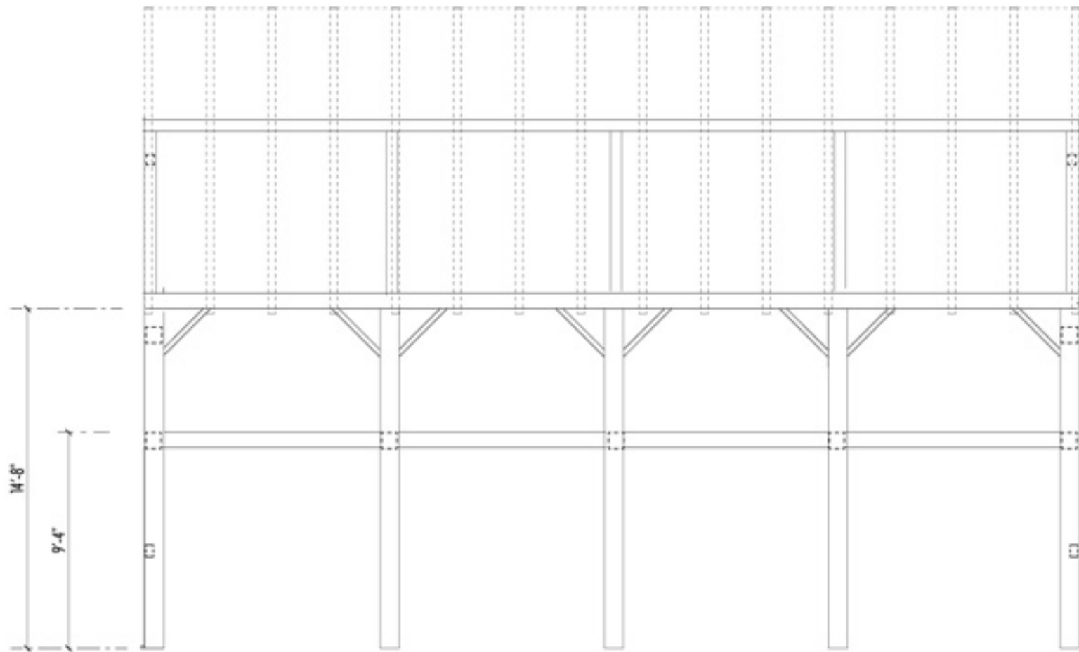
WEST EYE WALL C-C SCALE: 3/16" = 1'-0"
