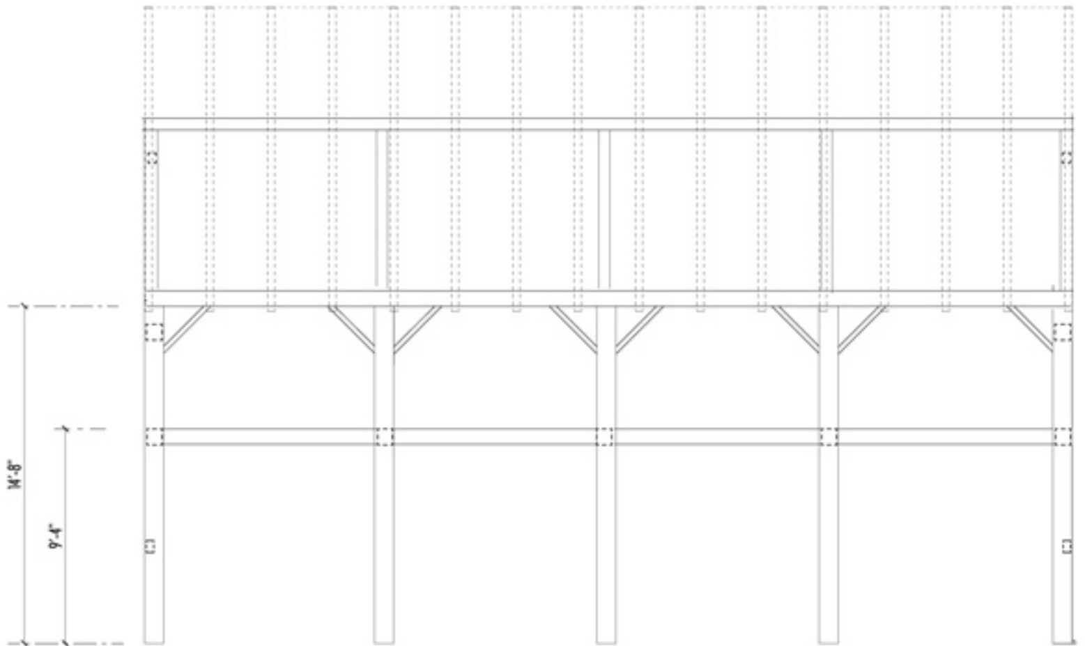
EAST EYE WALL D-D SCALE: 3/16" = 1'-0"
