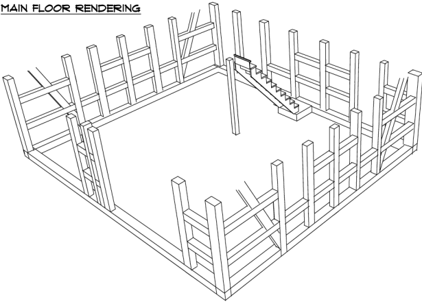
MAIN FLOOR RENDERING
